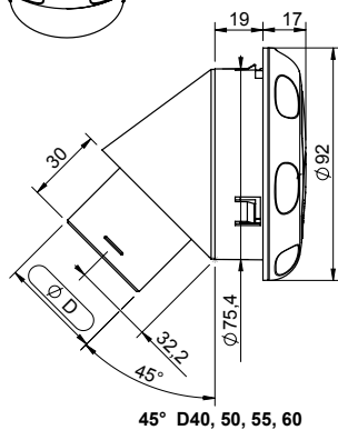
45° D40, 50, 55, 60
