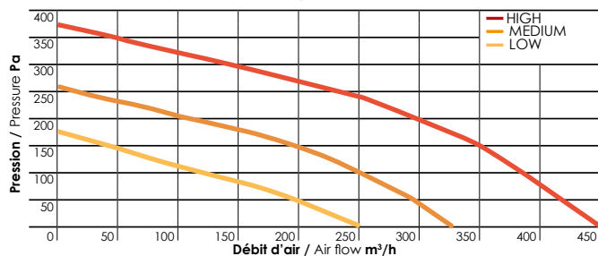
COURBE DÉBIT PRESSION / AIR FLOW PRESSURE CURVE
